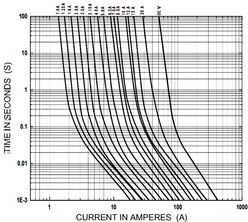
8-3 I-t图/CHARACTERISTICS DIAGRAM(I-t)
