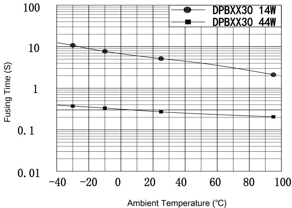
5-4 不同功率/环境温度下熔断时间曲线/FUSING TIME CURVE UNDER DIFFERENT POWER / AMBIENT TEMPERATURE
