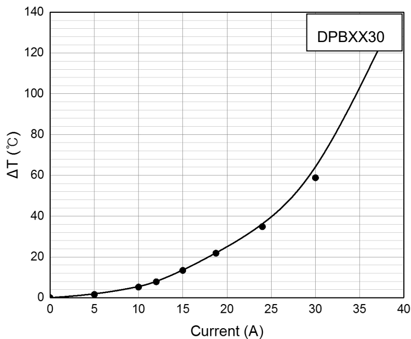
5-6 不同温度下的额定电流折算曲线/Rated current conversion curve at different temperatures
