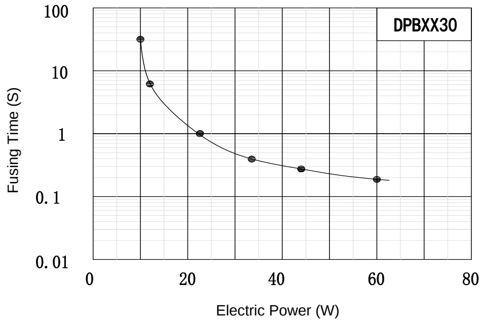
5-3 加热体功率与熔断时间曲线图/CURVE OF HEATING ELEMENT POWER AND FUSING TIME
